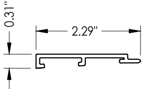
17 OUTSWING SIDELITE ADAPTER
