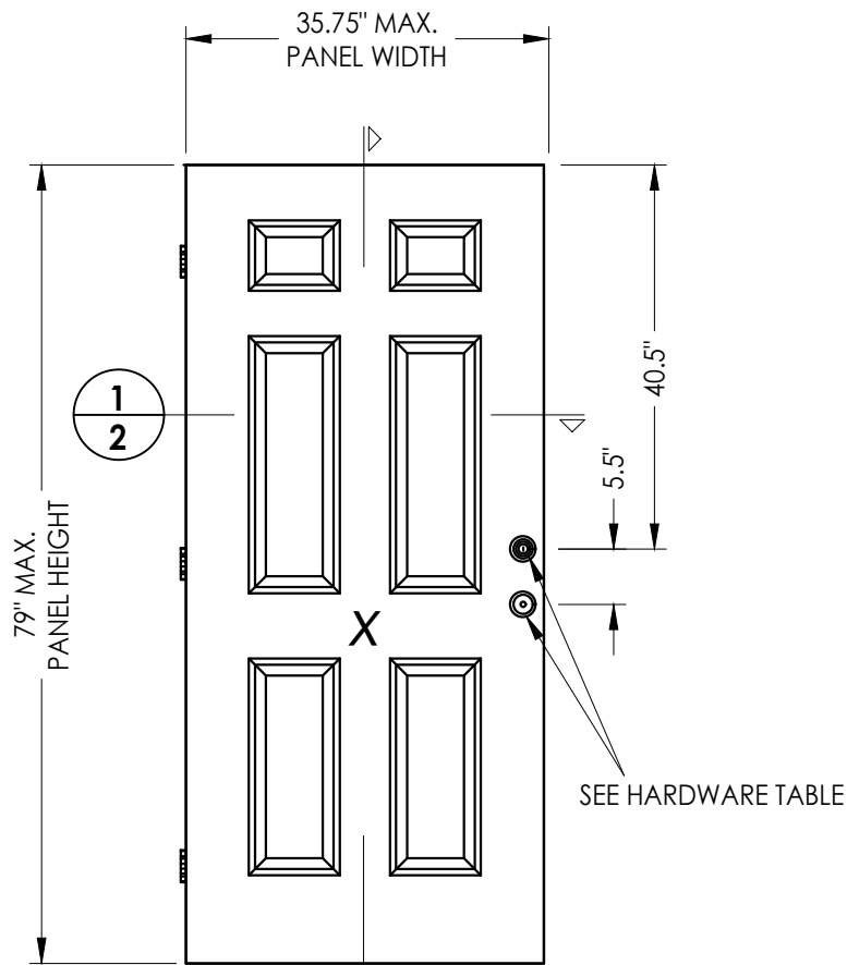
2 2 FIBERGLASS DOOR PANEL
