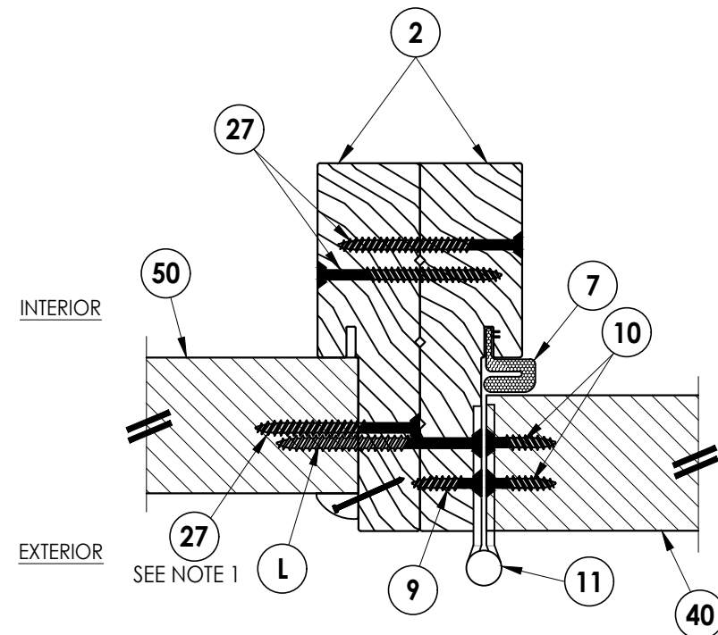
3 HORIZONTAL CROSS SECTION 5 Outswing Shown (Inswing Similar) Shown w/ Wood Jambs
