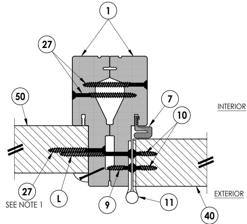
2 HORIZONTAL CROSS SECTION 5 Outswing Shown (Inswing Similar) Shown w/ PVC Jamb
