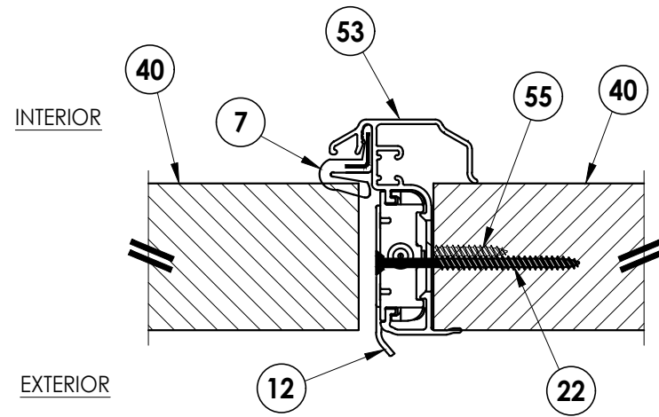
1 HORIZONTAL CROSS SECTION 5 Outswing Shown (Inswing Similar)
